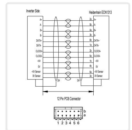
> Encoder Connection Terminal
