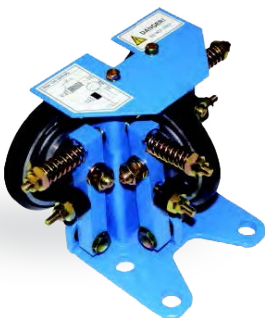
➤ ROLLER GUIDES
