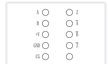
> Encoder Connection Terminal
