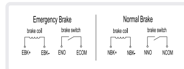
> Brake Wiring Diagram for TMGL-B
