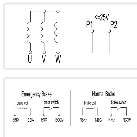
> Brake Wiring Diagram
