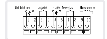
> Sheave Clamp Wiring Diagram
