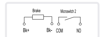
> Sheave Brake Wiring Diagram
