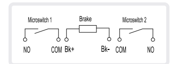
> Normal Brake Wiring Diagram
