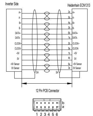
> Encoder Connection Terminal
